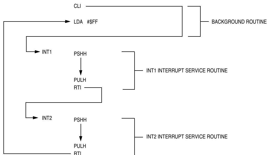
Figure 7-11. Interrupt Recognition Example
