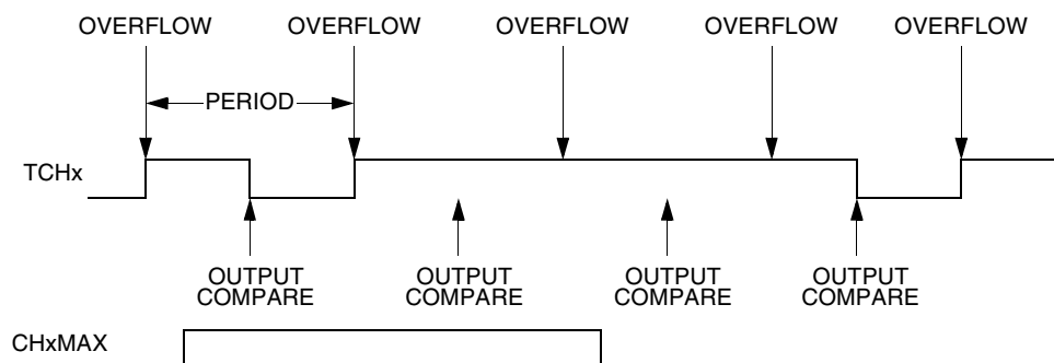
Figure 10-11. CHxMAX Latency
