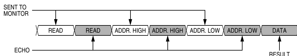
Figure 9-5. Read Transaction
