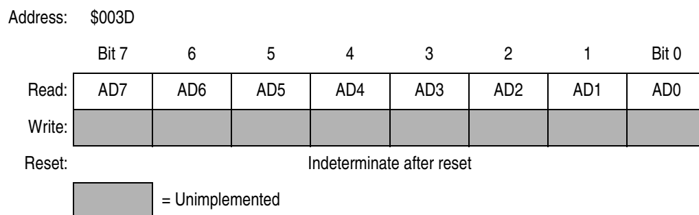
Figure 12-4. ADC Data Register (ADR)
