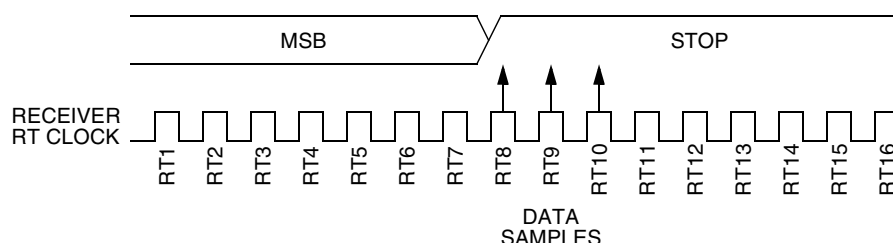
Figure 11-7. Slow Data
