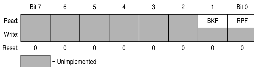
Figure 11-14. SCI Status Register 2 (SCS2)
